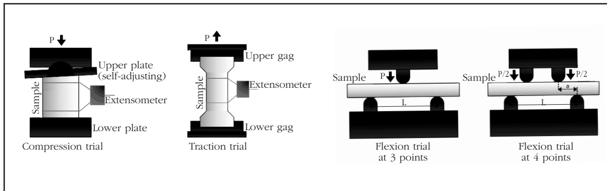
Figure 5. Schematic representation of the principal classic mechanical trials
