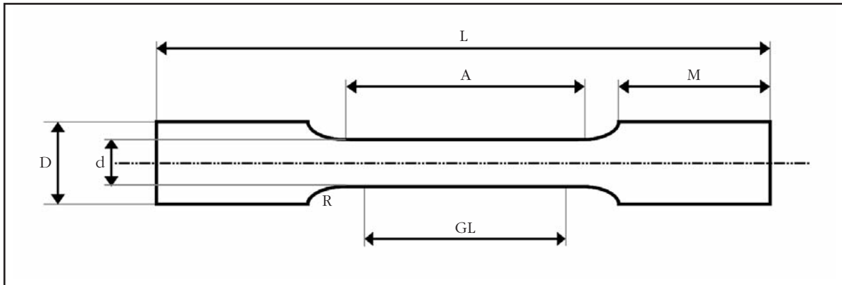
Figure 4. Geometry of a sample for a traction test. L: total length; A: parallel length; GL: calibrated length; M: end length; D: diameter of the sample at the ends; d diameter of the sample in the test area; R: radius of curvature
