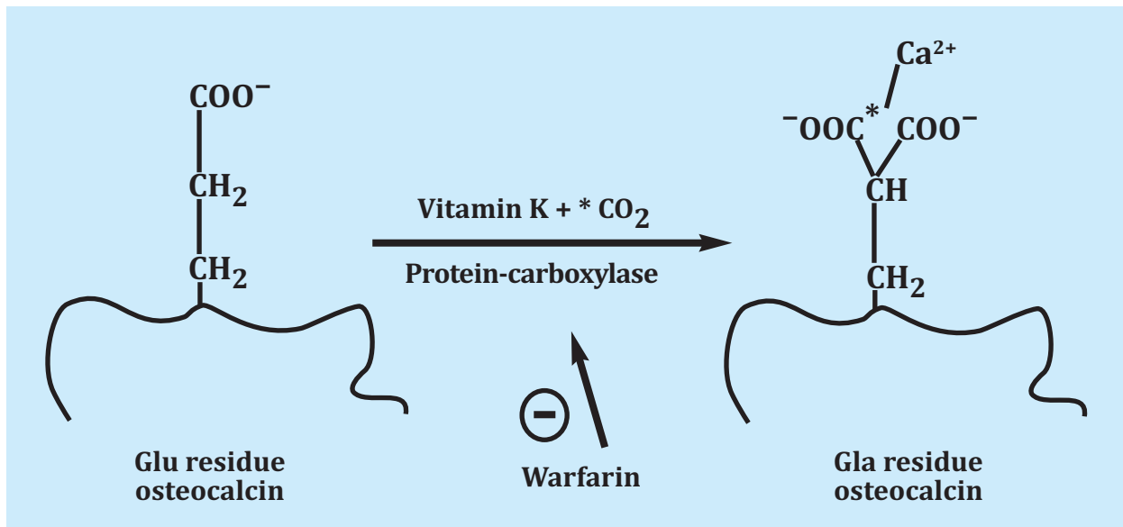
Figure 1. By post-translational carboxylation, the glutamic acid of osteocalcin is transformed into gamma-carboxyglutamic acid. The presence of the two carboxyl groups causes a high affinity for the calcium \text{Ca}^{2+} binding of the extracellular matrix
